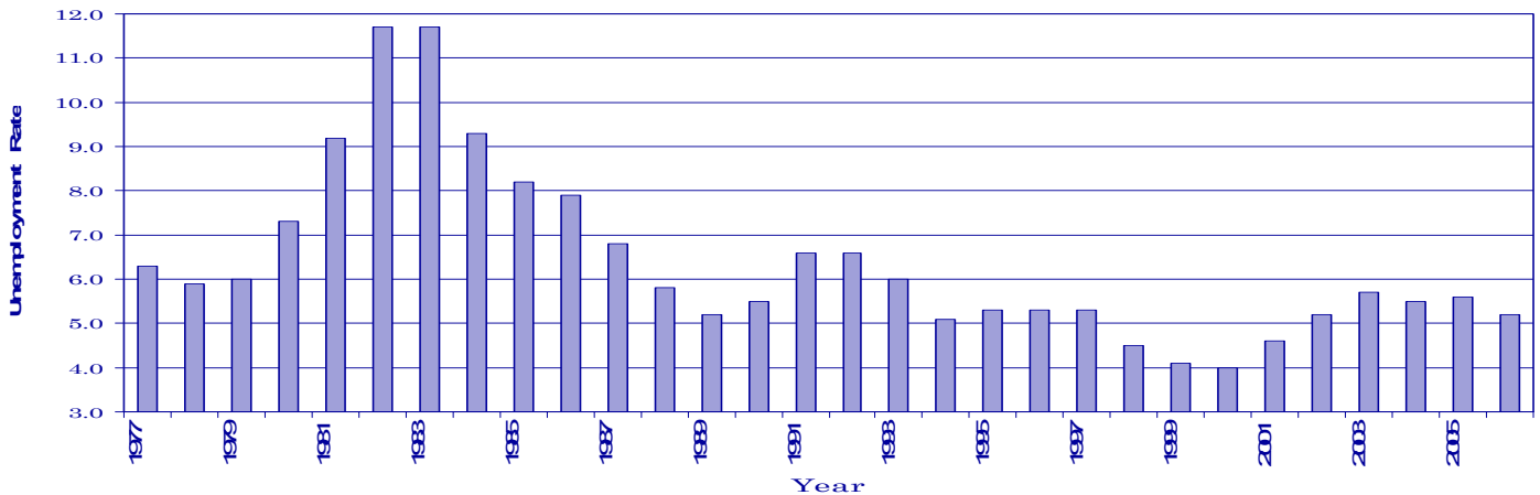
Unemployment Rates 1977-2006
