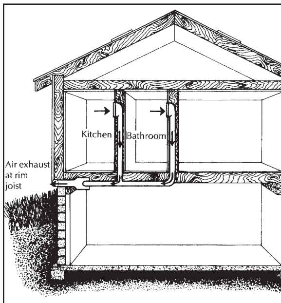
Figure 4 Mechanical ventilation
