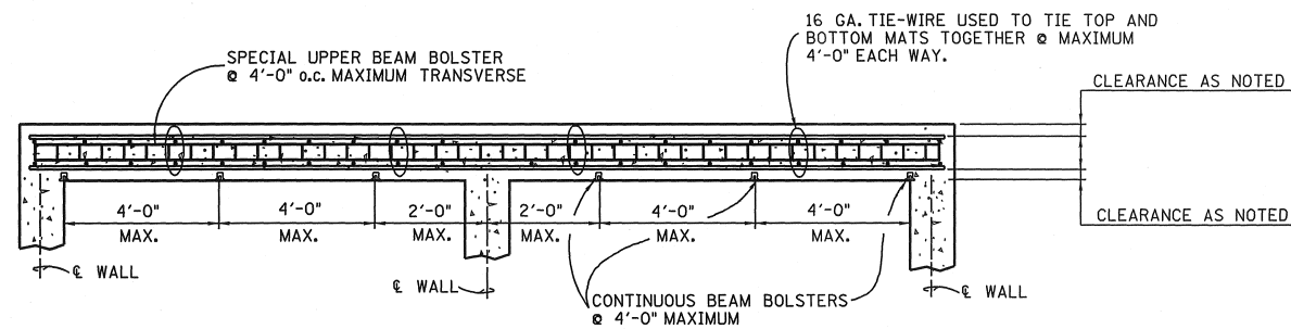
▲ TYPICAL DETAILS FOR BOX TYPE STRUCTURES
