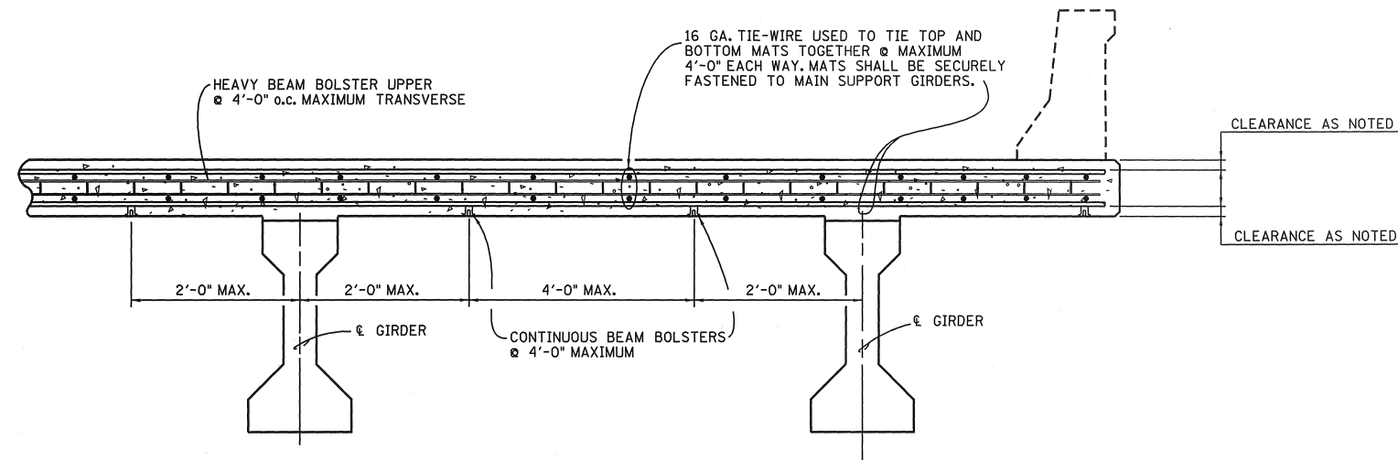
▲ TYPICAL DETAILS FOR GIRDER TYPE BRIDGES
