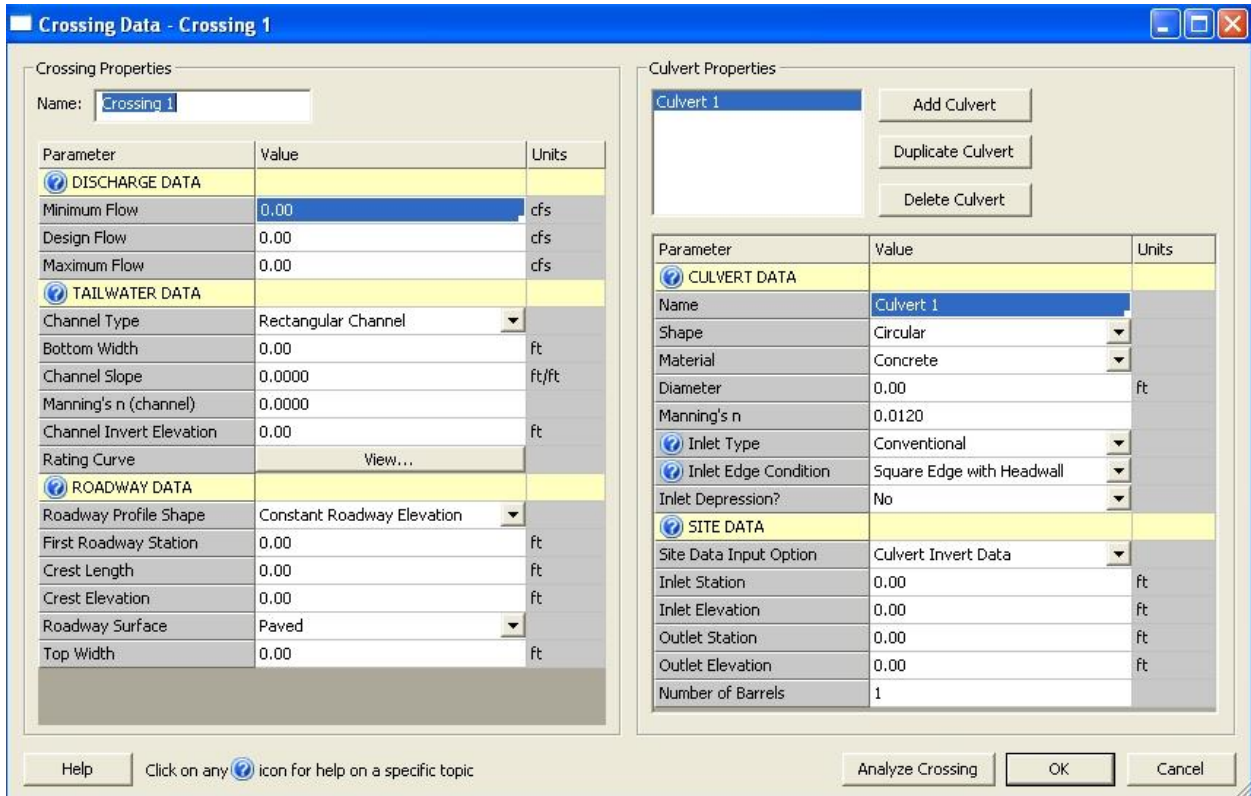
Figure 6A-16 HY-8 Data Input Screen
