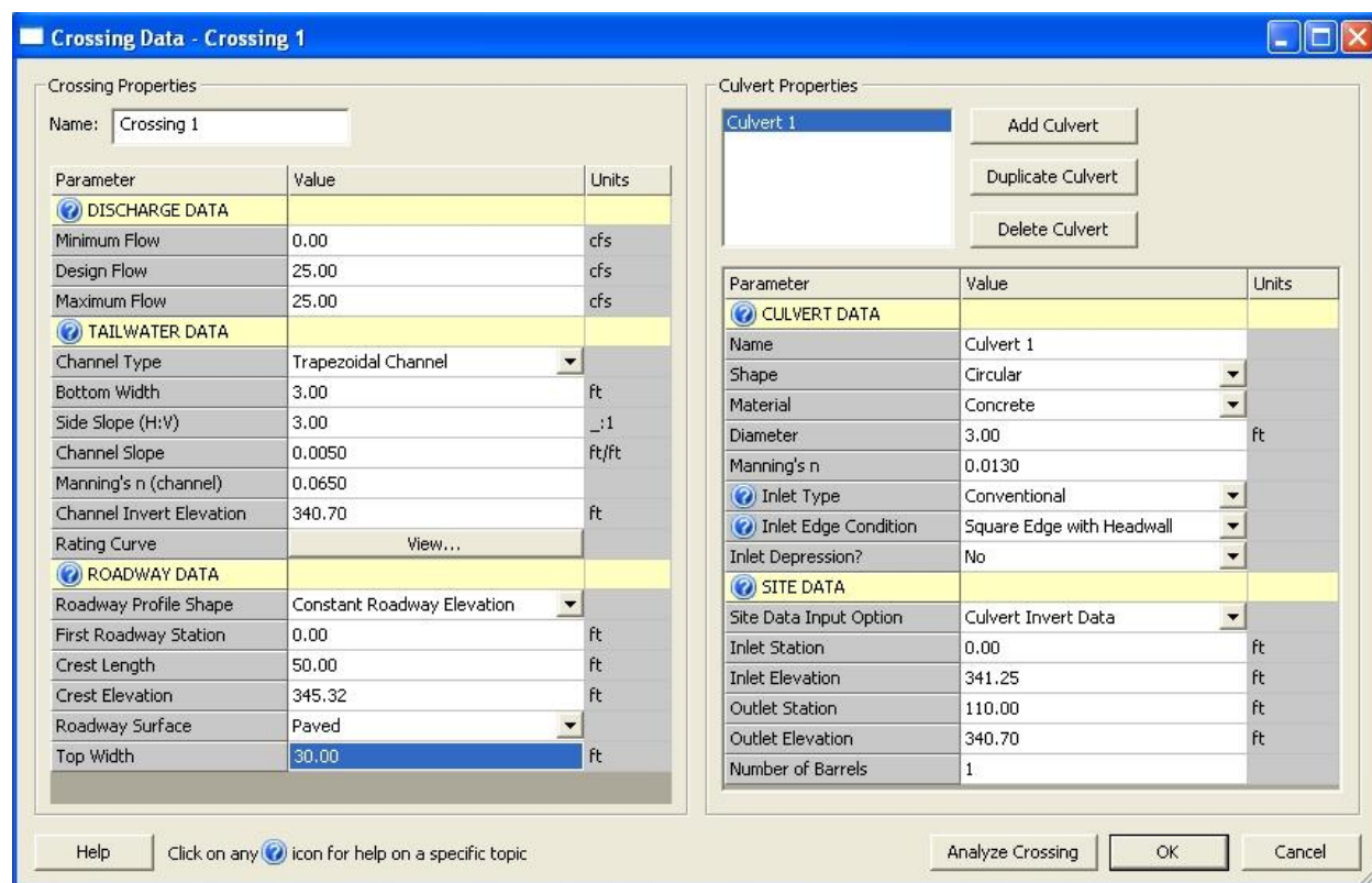
Figure 6A-21 HY-8 Data Summary Screen
