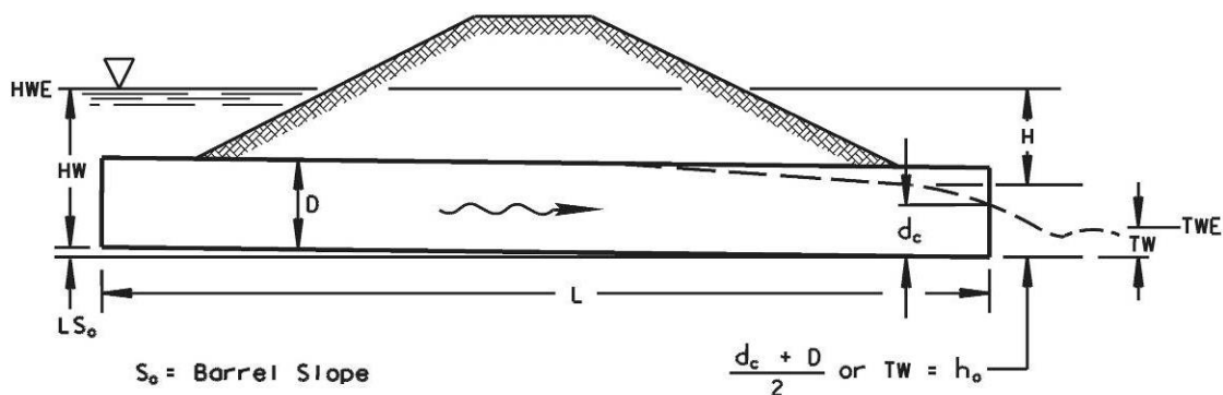
Figure 6-10 Outlet Control Headwater Depth H_{w_o}
