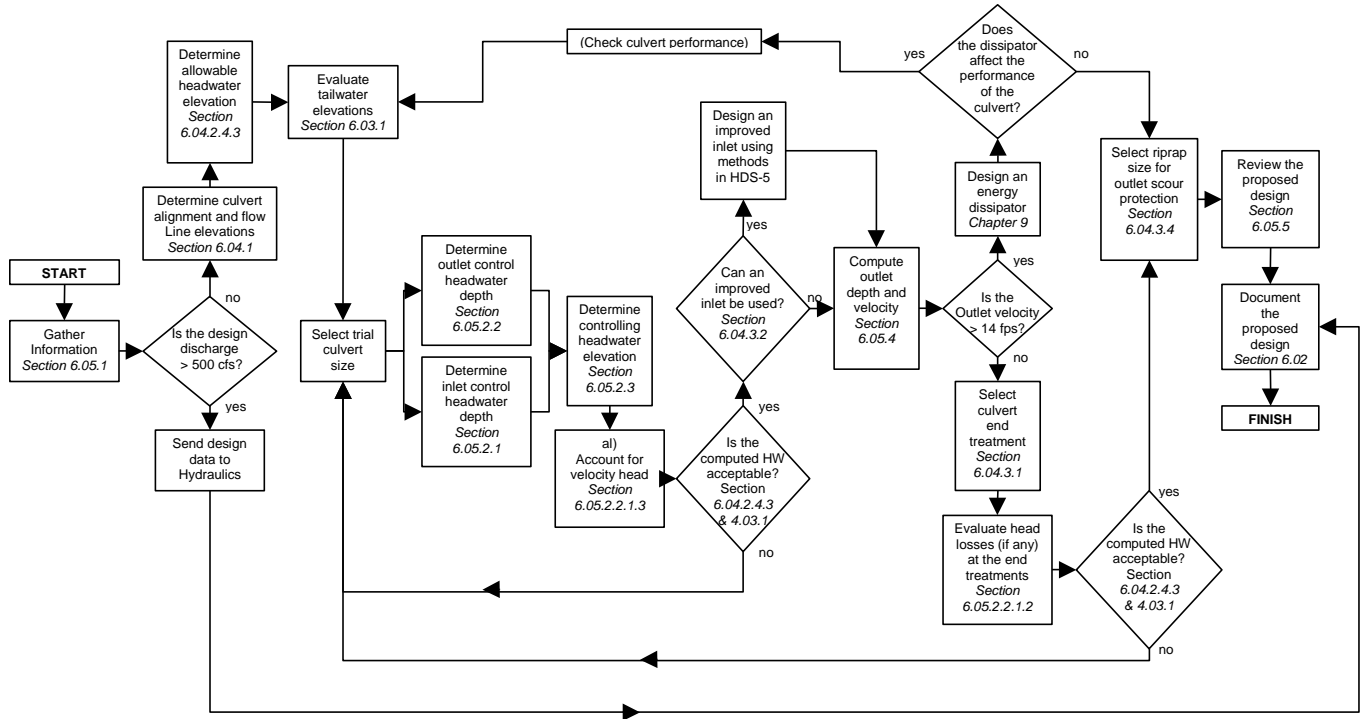
Figure 6A-1 Culvert Design Flow Chart
