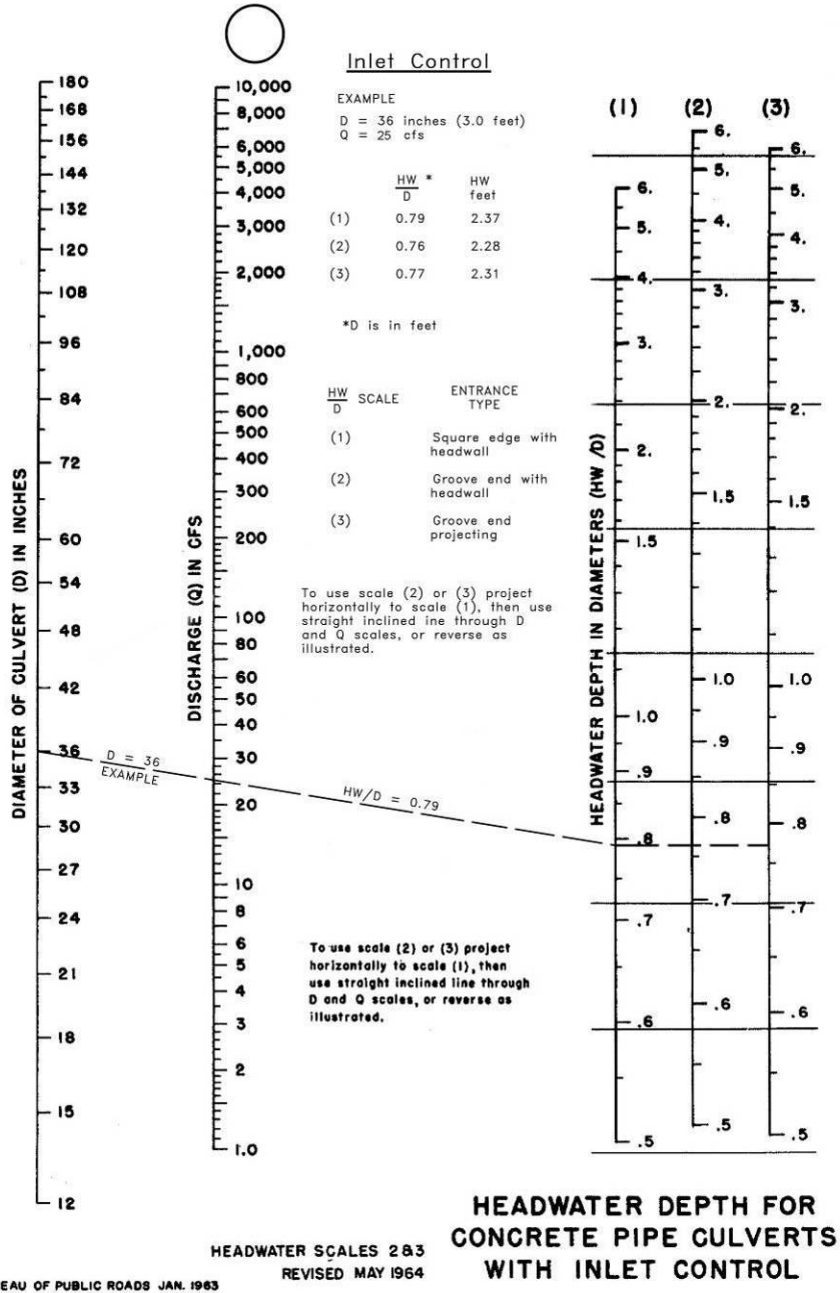
Figure 6A-13 Completed Inlet Control Headwater Chart (Problem #1) Reference: USDOT, FHWA, HDS-5 (1985)
