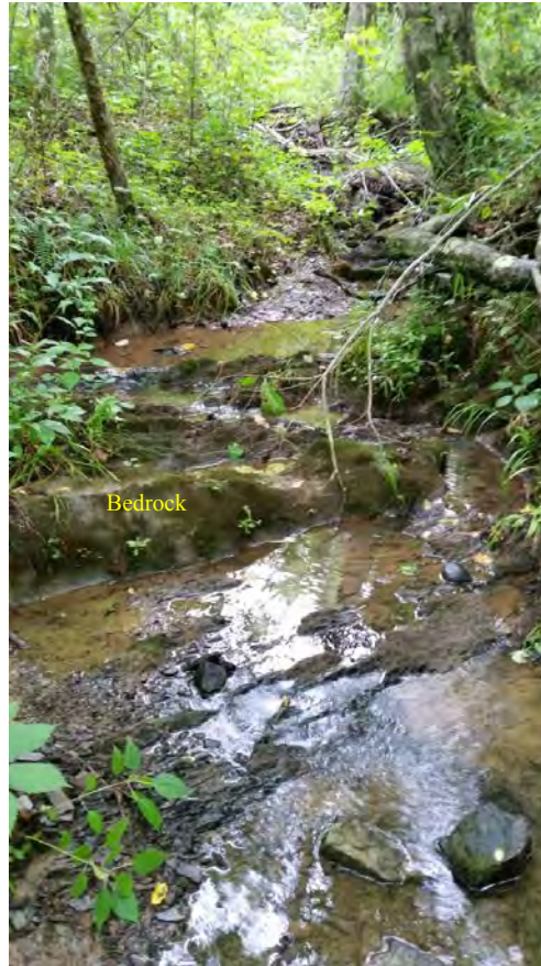
Fig. 8. Nolichucky Shale outcrop in NT-11 stream channel.
