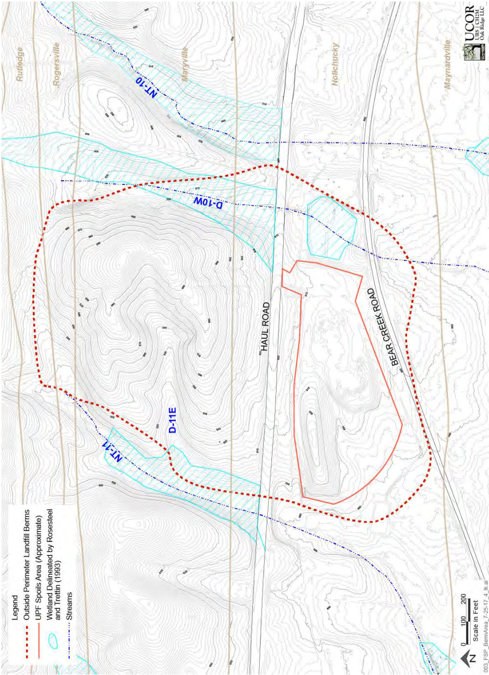
Fig. 2. CBCV site topographic setting.
