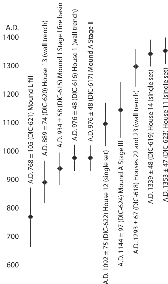
Figure 17. Calibrated radiocarbon dates from Mound Bottom. Assays were calibrated using CalPal 2007. We urge caution in using these dates for anything more than approximations (see text for explanation).
