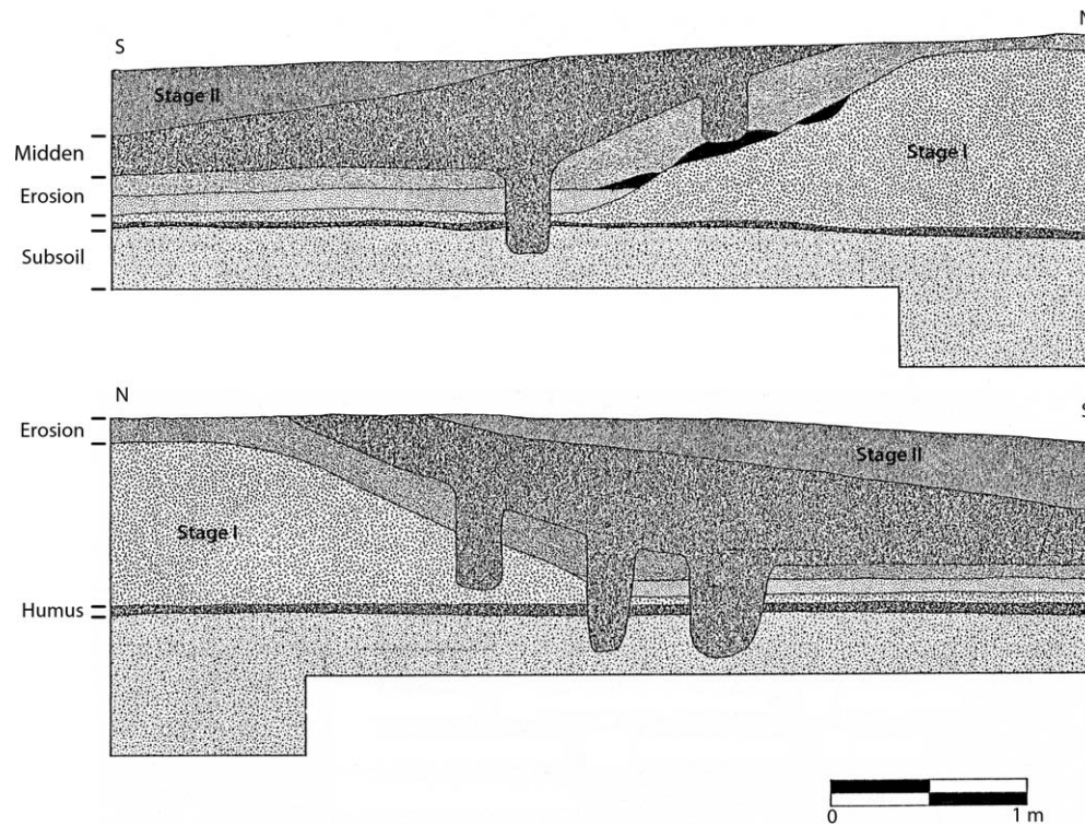
Figure 8. Profiles of the 5- \times -5-m unit on the southern flank of Mound J: (top) west profile showing both stages of mound construction, intervening midden and slope wash, and two large post molds; (bottom) east profile showing the same stratigraphic units and three post molds. Note the remains of three logs (shown in black) in the west profile possibly representing steps.
